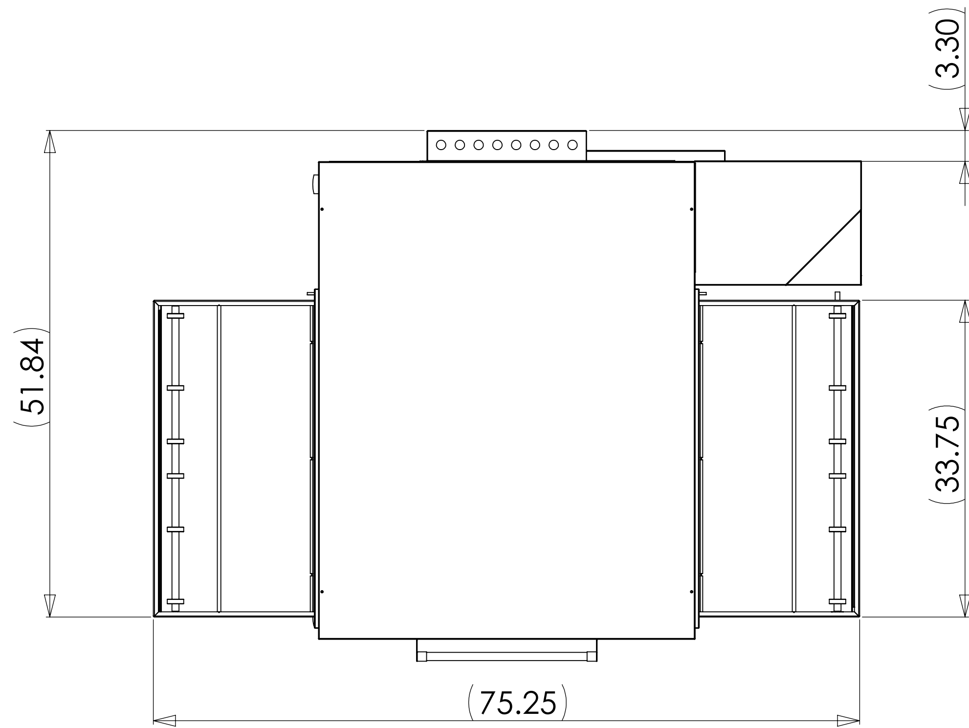
TOP VIEW
