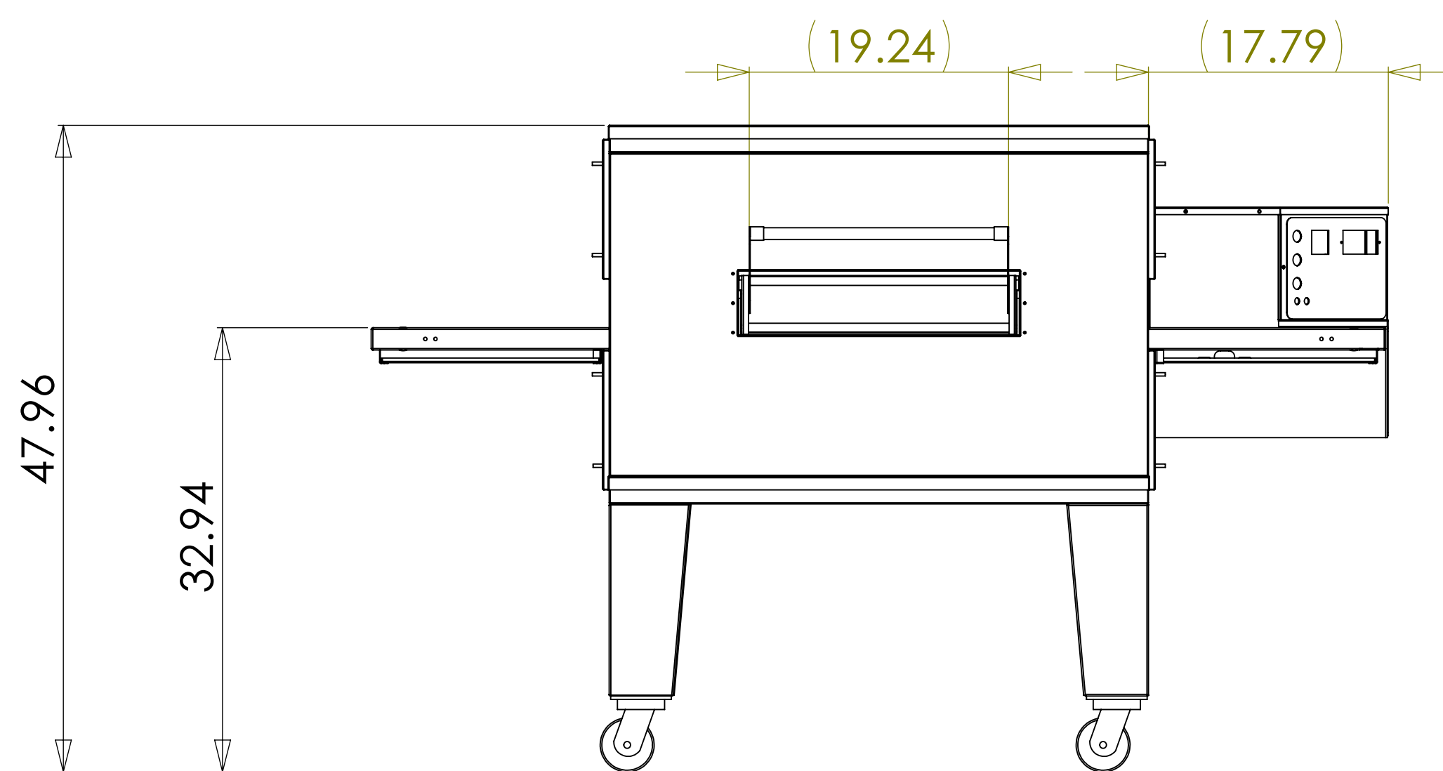
FRONT VIEW
