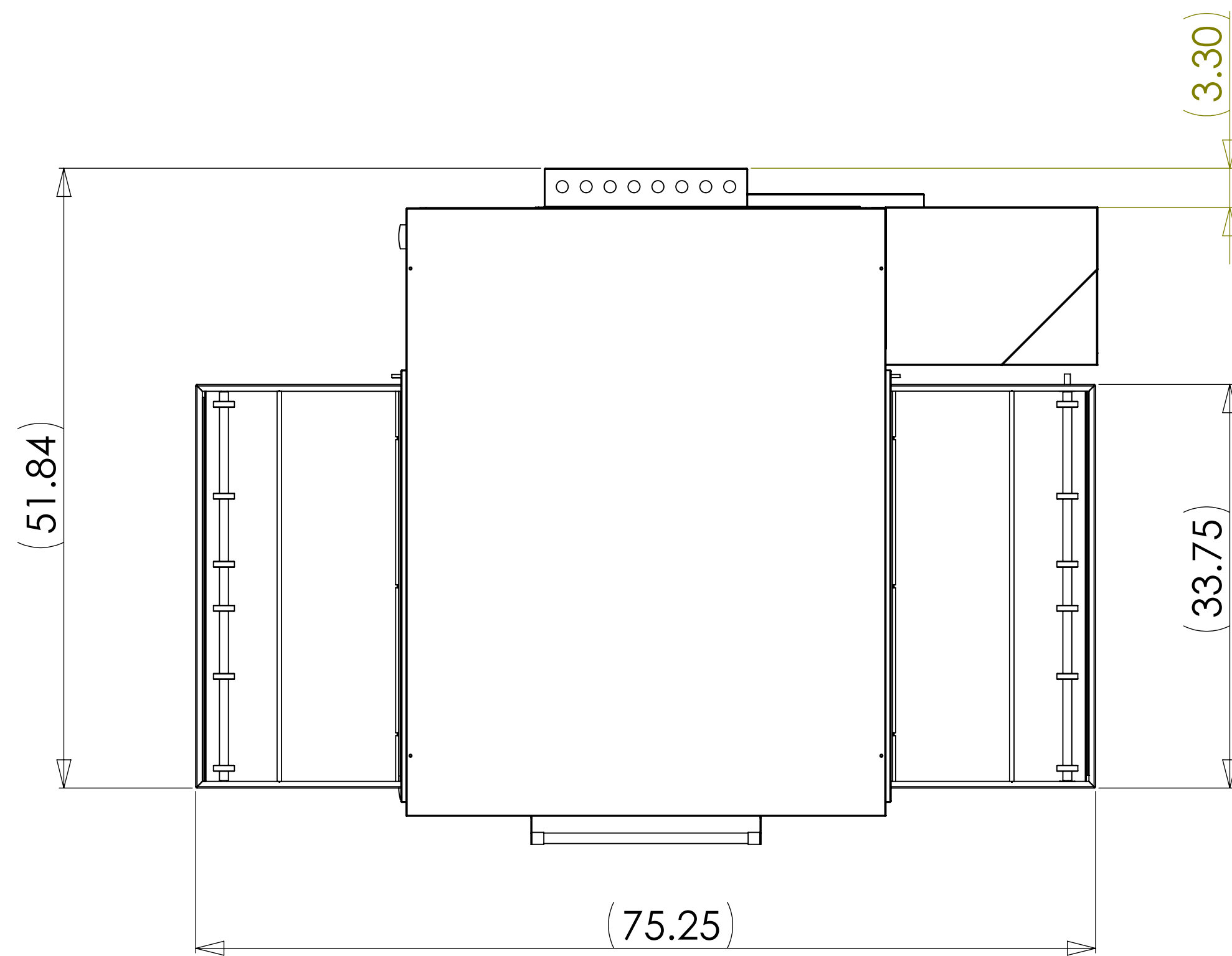
TOP VIEW
