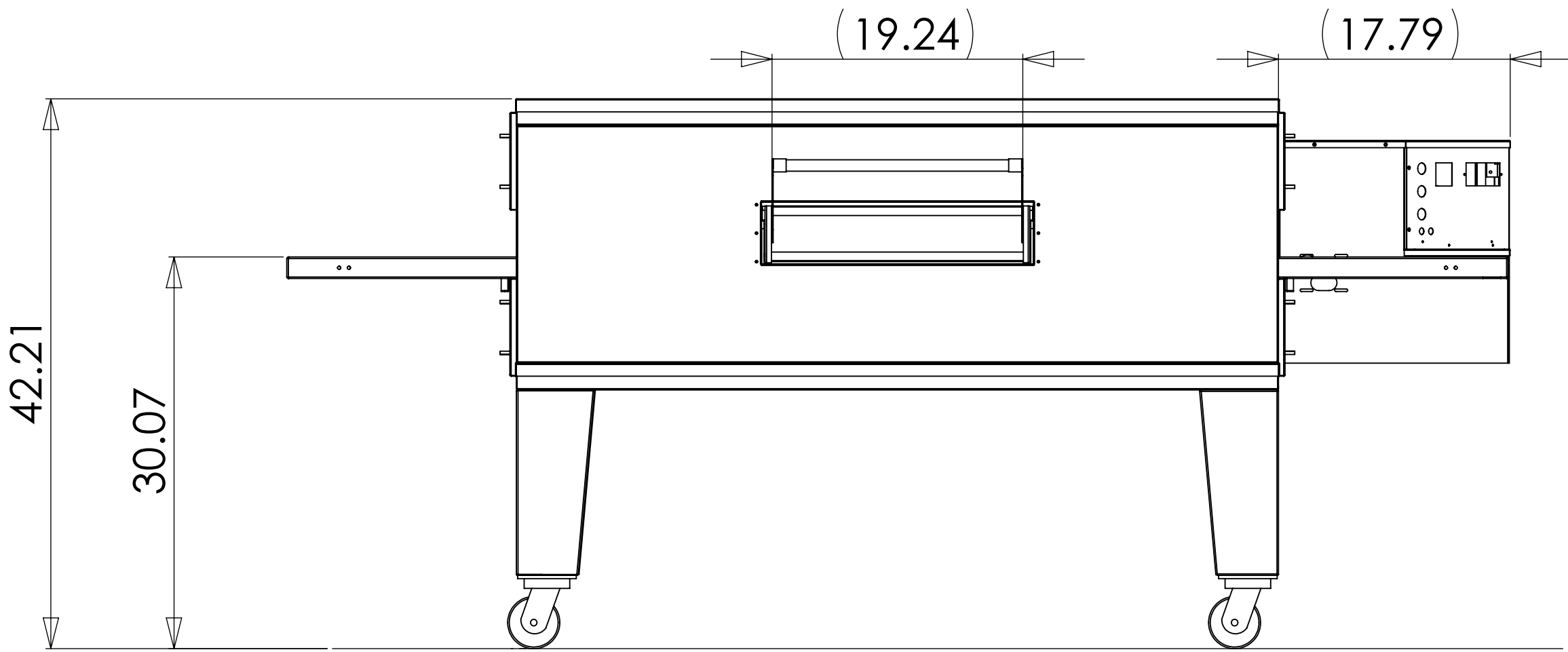
FRONT VIEW
